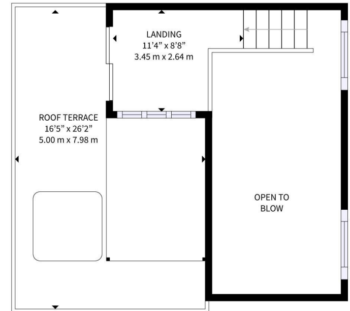
FLOOR 3
